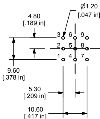
PCB LAYOUT
